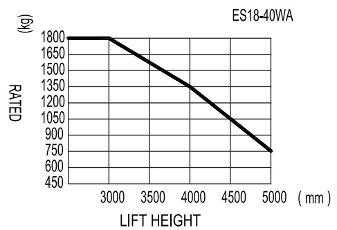
RATED CAPACITIES GRAPH
